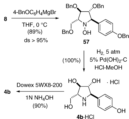
Scheme 12. Synthesis of radicamine B.
