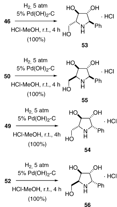
Scheme 11. Synthesis of 2-phenyl-substituted polyhydroxylated pyrrolidines.
