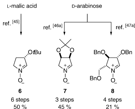
Scheme 2. Synthesis of cyclic nitrones.
