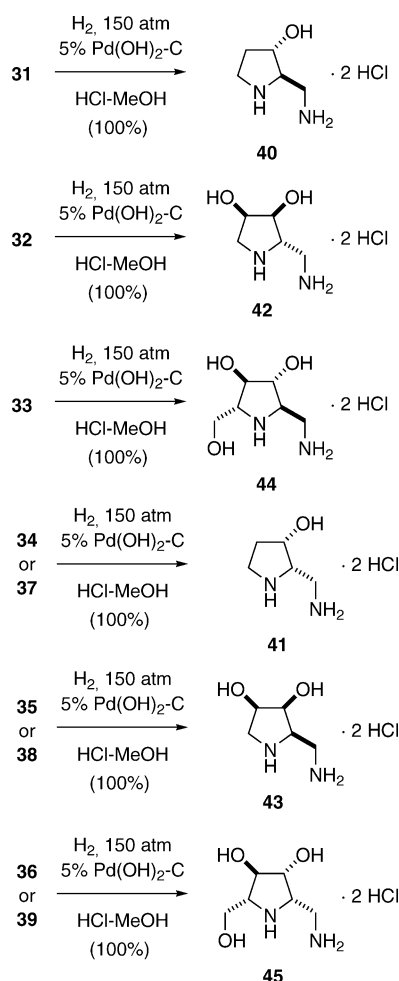
Scheme 9. Synthesis of 2-(aminomethyl)pyrrolidines.
