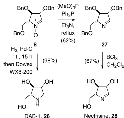
Scheme 6. Syntheses of DAB-1 and nectrisine.
