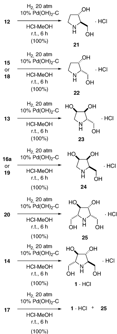
Scheme 5. Hydrogenation/deprotection of protected hydroxylamines.
