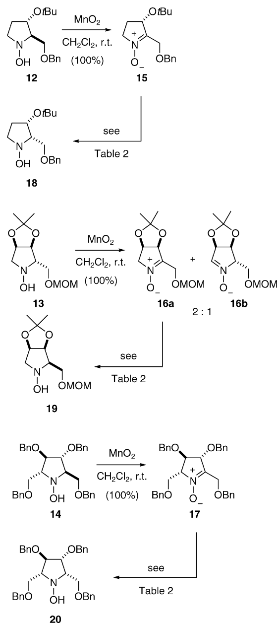
Scheme 4. Oxidation and reduction of cyclic hydroxylamines.
