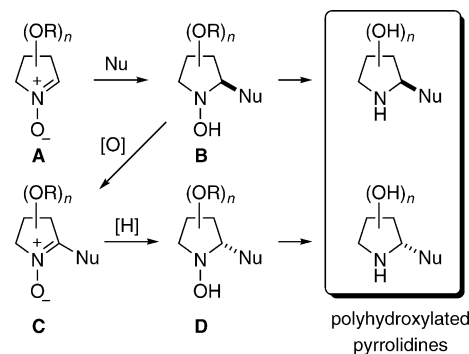
Scheme 1. Synthetic plan.
