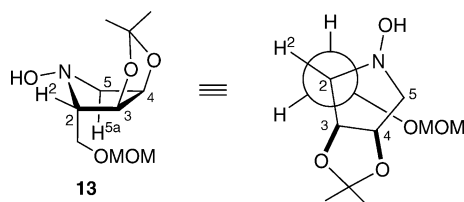
Figure 2. Antiperiplanar 2-H/OMOM conformation in 13 .
