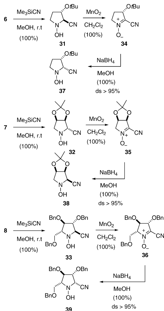
Scheme 8. Synthesis of 2-cyano- N -hydroxypyrrolidines.
