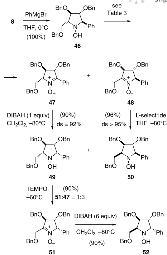
Scheme 10. Synthesis of protected 1-hydroxy-2-phenylpyrrolidines.
