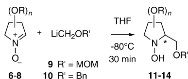
Scheme 3. Addition of protected hydroxymethyl lithium derivatives.
