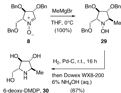
Scheme 7. Synthesis of 6-deoxy-DMDP.
