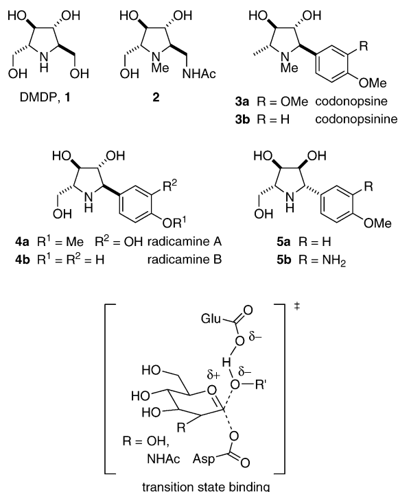
Figure 1. Polyhydroxylated pyrrolidines as inhibitors of glycosidases.
